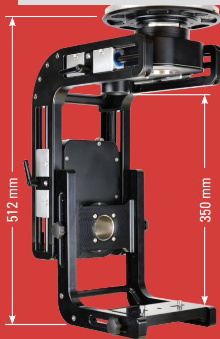
MEDIUM SETTING
